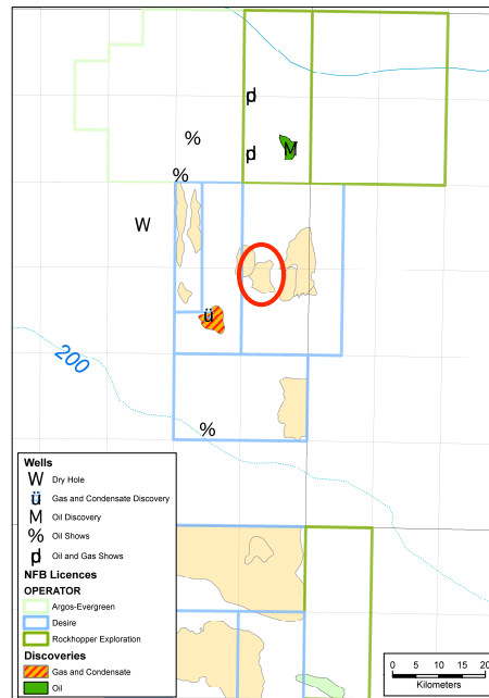
Lower F3 sand: Maximum Amplitude
