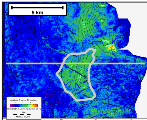
Lower F3 sand: Maximum Amplitude
