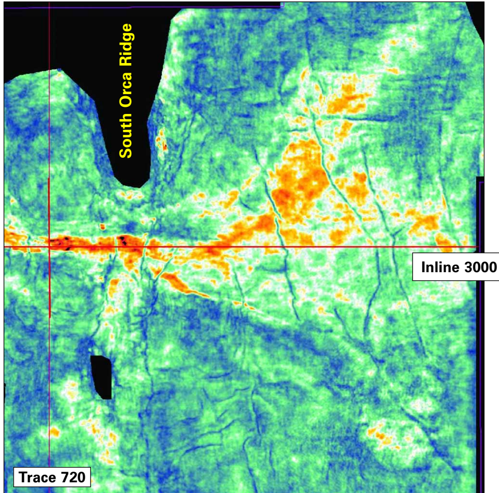
Seismic amplitude map suggests a major fan-delta, at the level of the mature oil source rock
