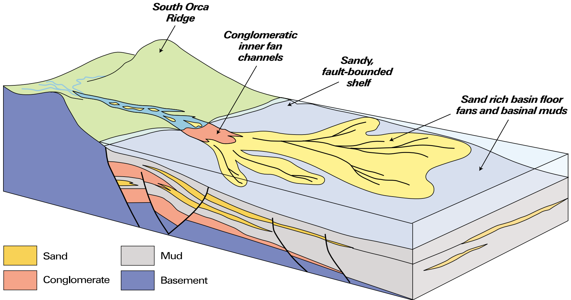
Schematic illustration of the Environment of Deposition in the Liz Prospect Area
